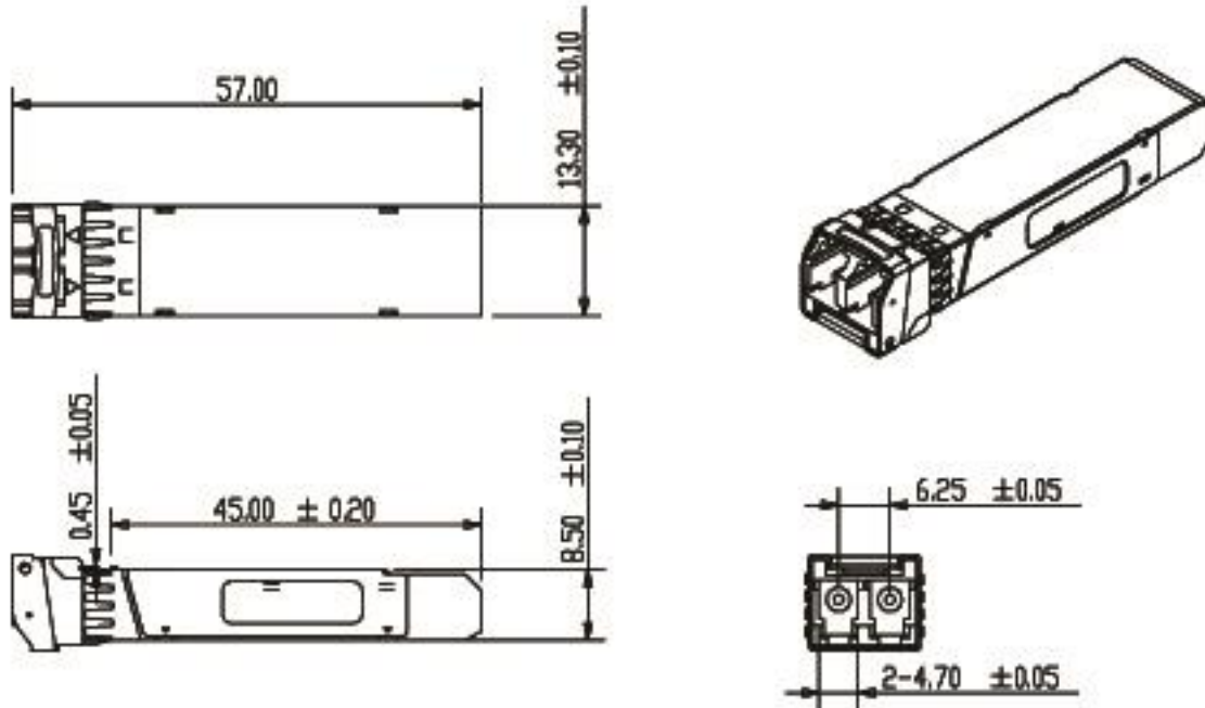
Figure5. Mechanical Dimensions
