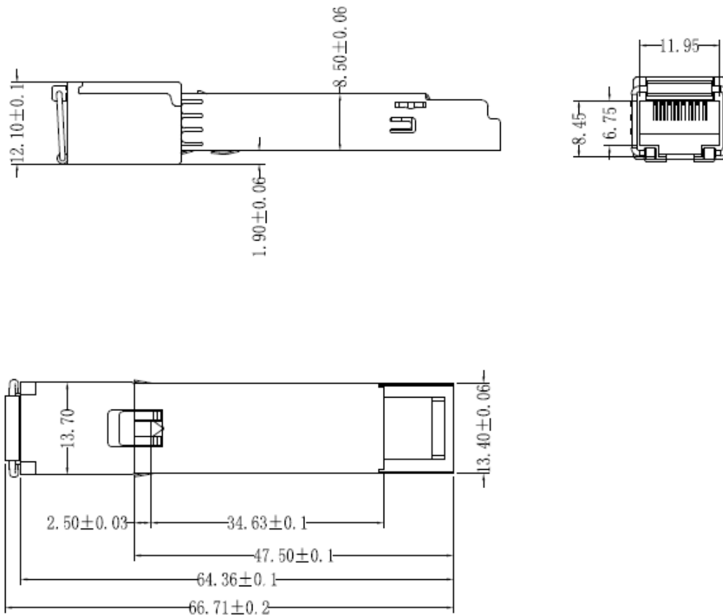
Figure 2. Mechanical dimensions
