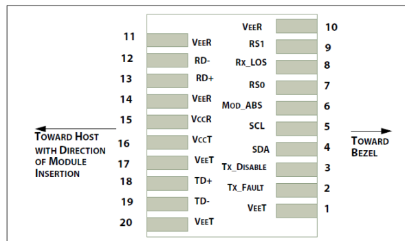
Figure 2. Module Interface to Host
