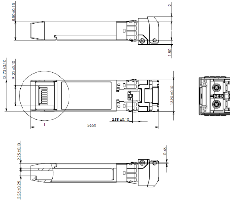
Figure 4. Mechanical Outline
