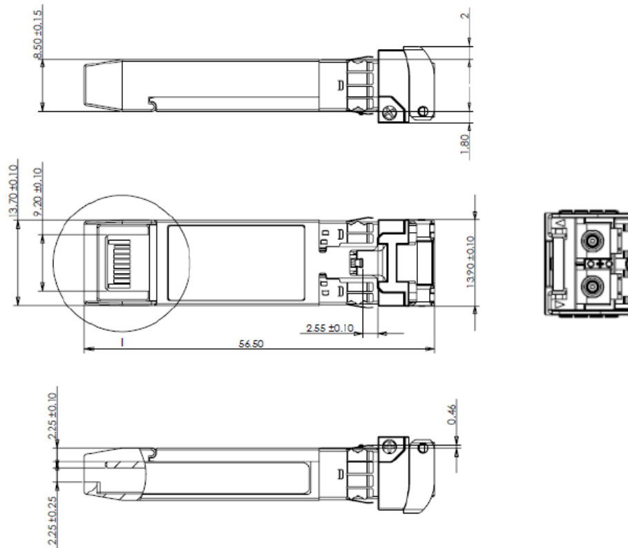
Figure 4. Mechanical Outline
