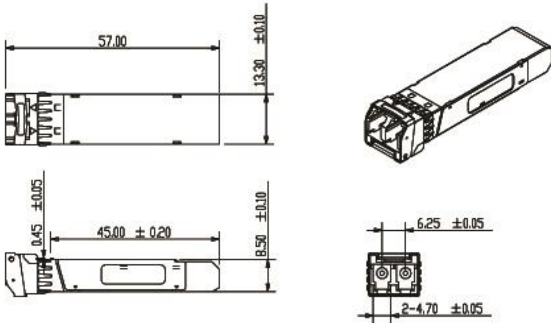
Figure6. Mechanical Specifications
